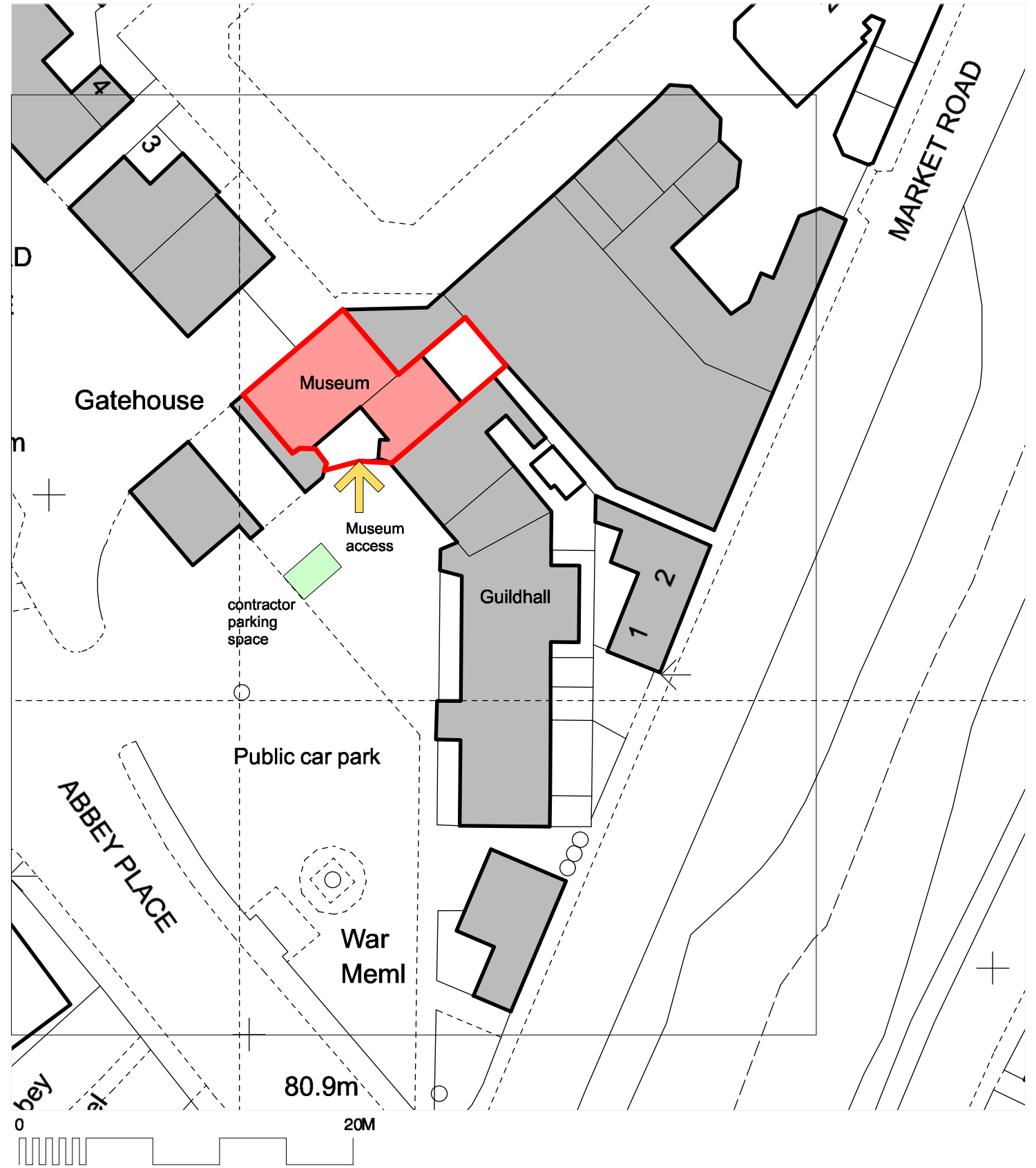
Block and access plan - scale 1:500@ A3
